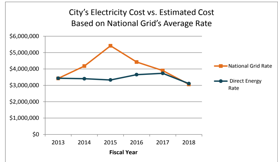
Figure 7: The graph provides a comparison of the City's actual electricity cost based on its third-party supplier rate versus estimated cost using National Grid's average rate.
