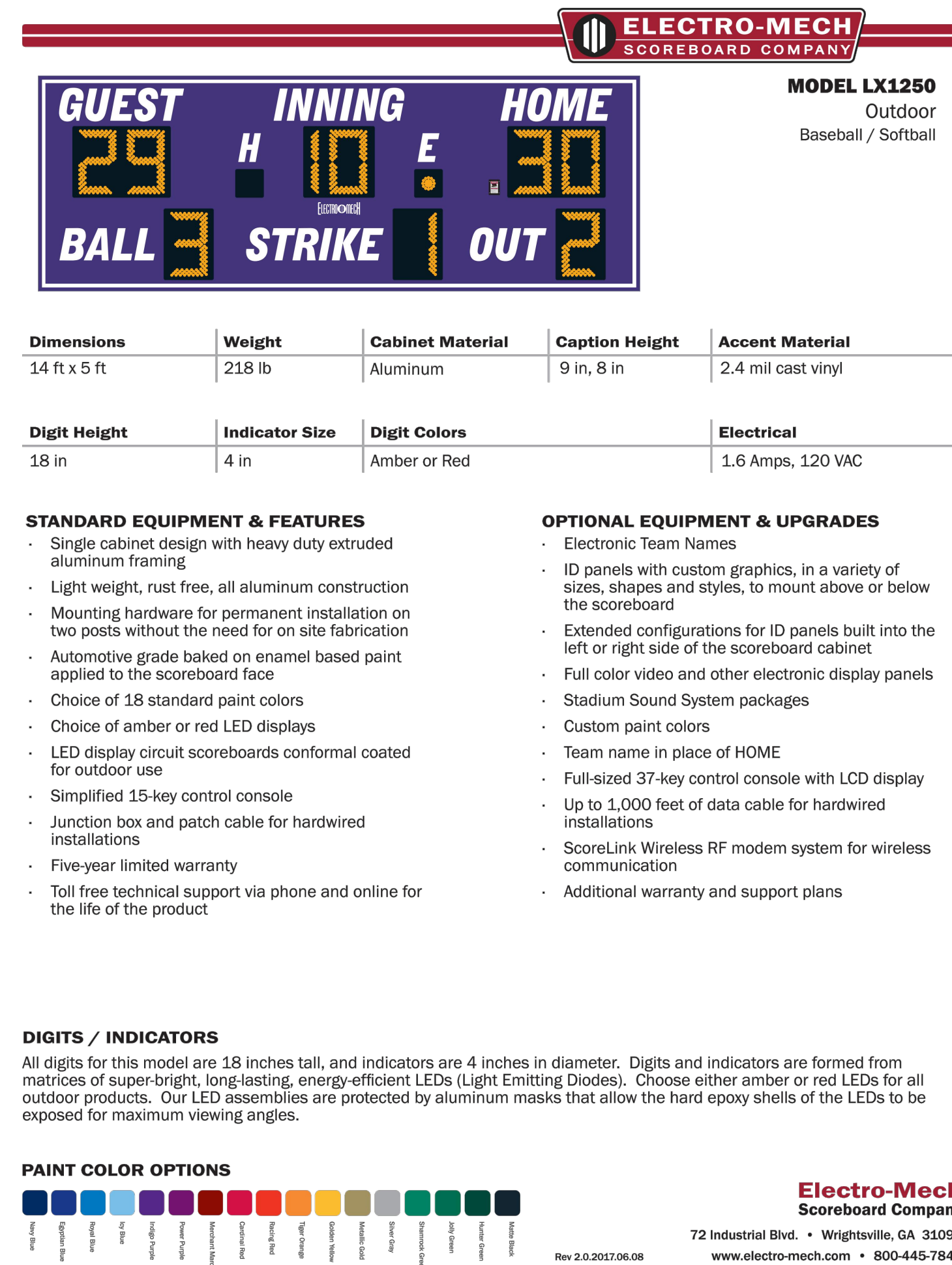
C SCOREBOARD SPECIFICATIONS
