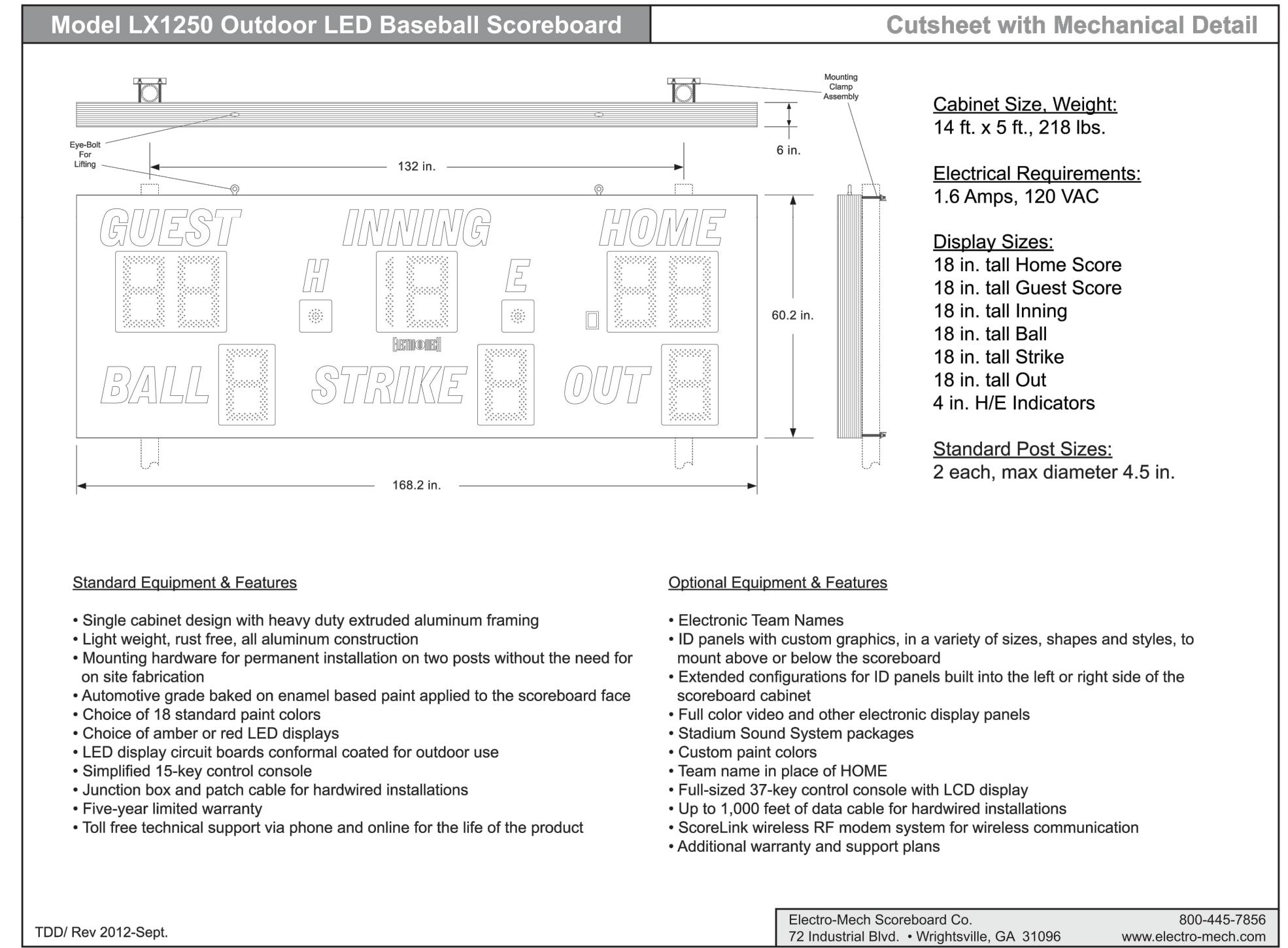
B SCOREBOARD CUTSHEET DETAIL
