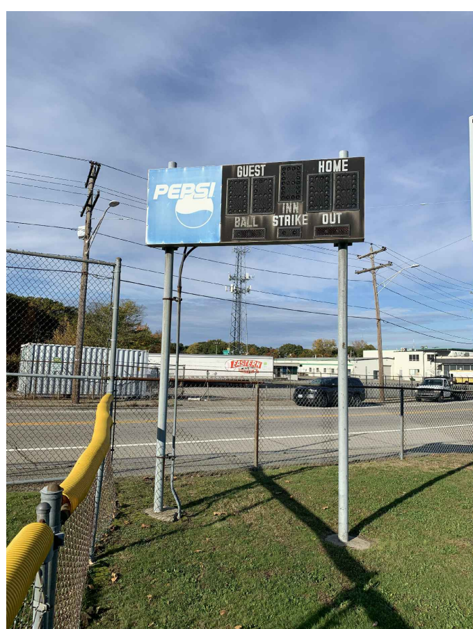
3 SOUTHERN FIELD SCOREBOARD 84.25" CENTER TO CENTER DISTANCE BETWEEN POLES
