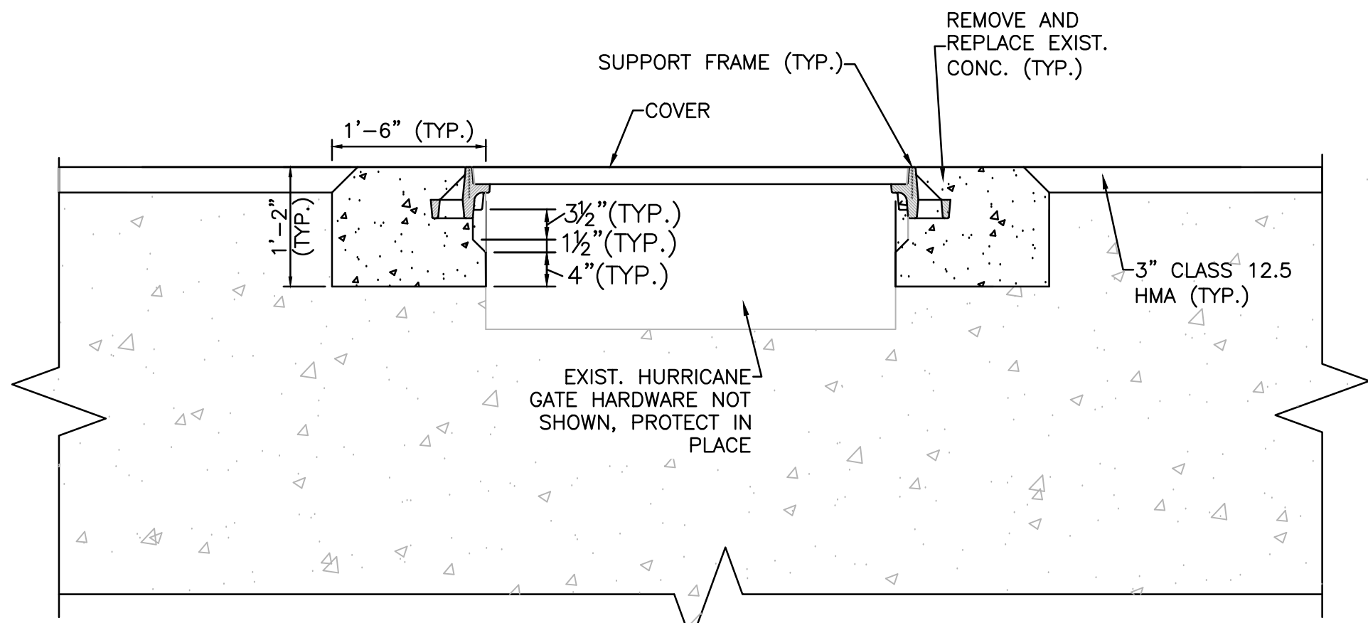
PROPOSED SECTION B SCALE: 3/4" = 1'-0"
