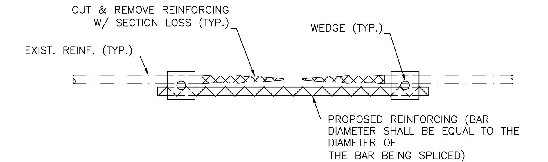
MECHANICAL COUPLER – OPTION 2
