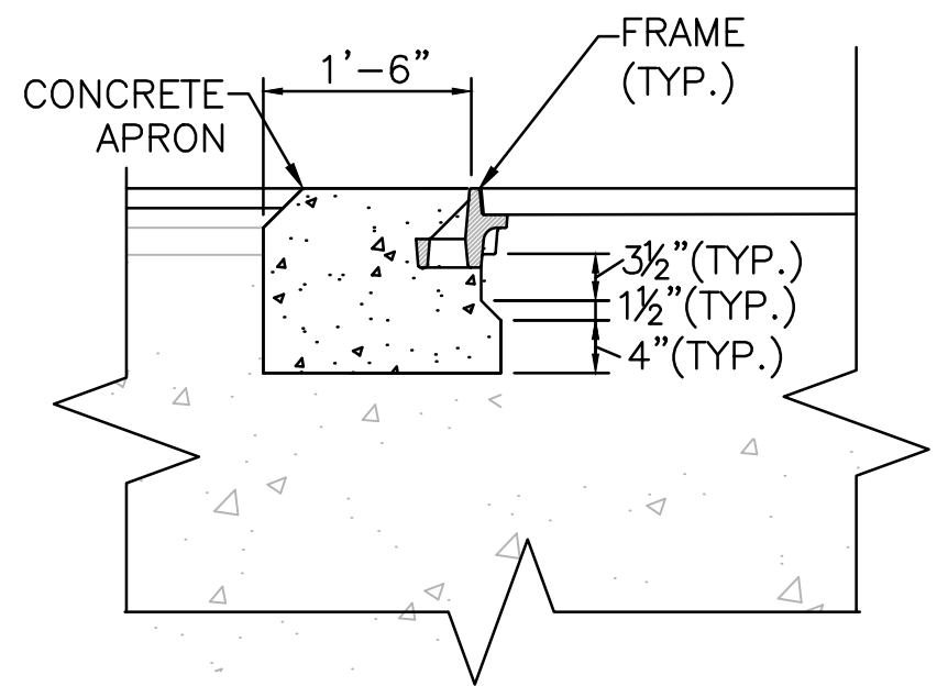
CONCRETE ADJUSTMENT DETAIL
