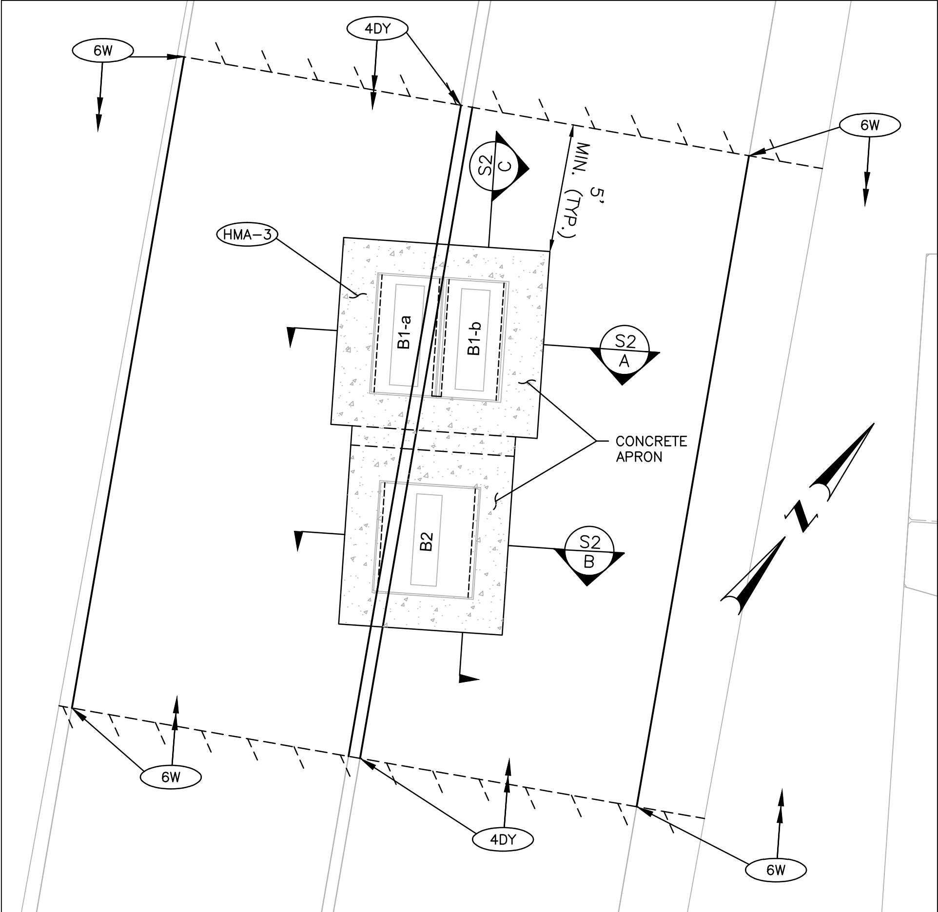
BRIDGE STREET SCALE: 1" = 4'
