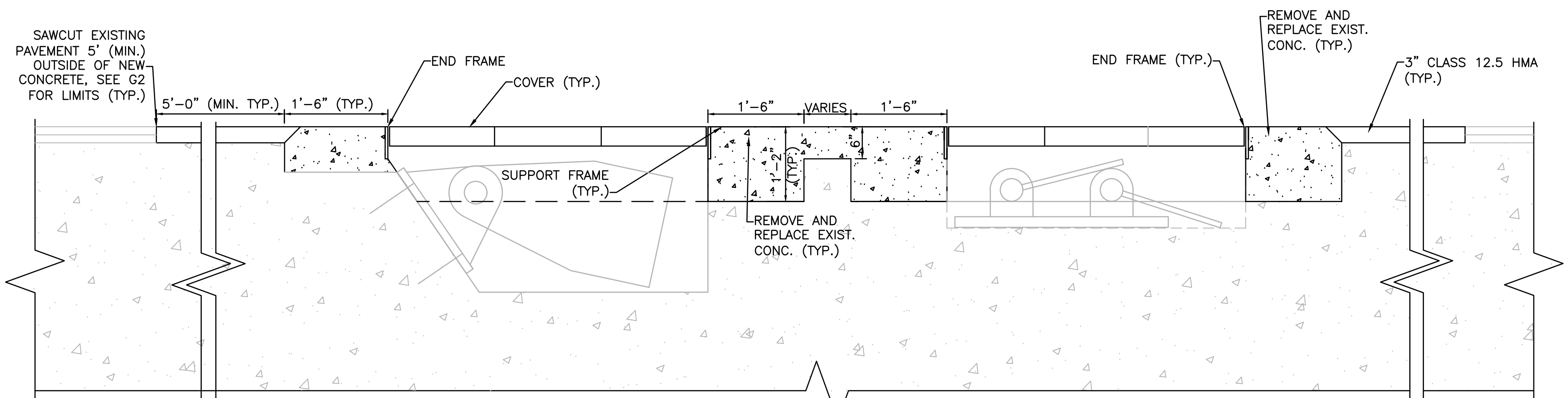
PROPOSED SECTION C SCALE: 3/4" = 1'-0"
