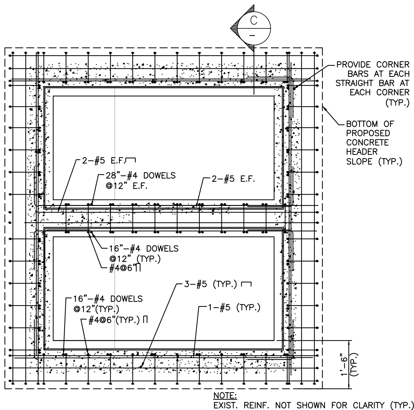
DETAIL CURB REINFORCING PLAN SCALE: NTS
