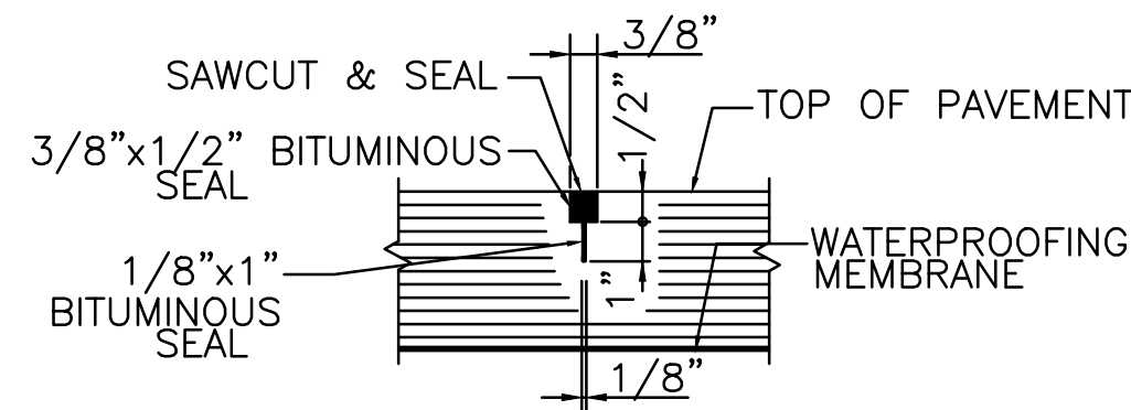
SAWCUT & SEAL DETAIL
