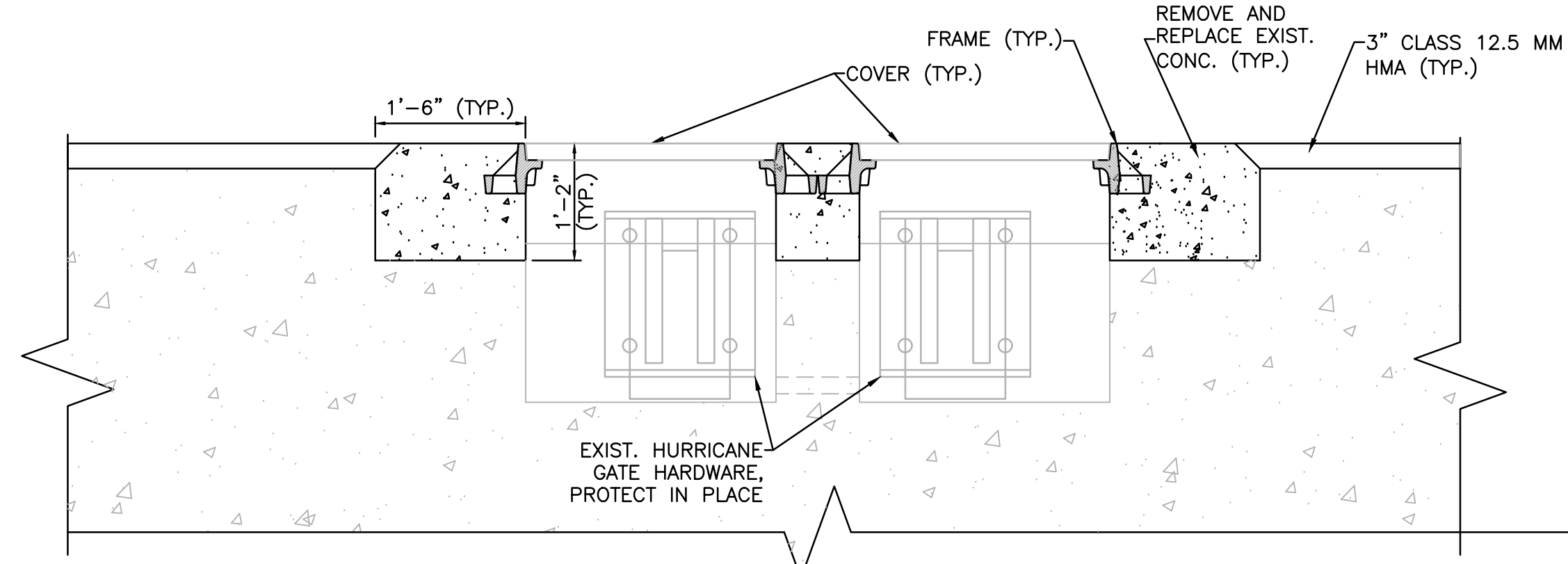
PROPOSED SECTION A SCALE: 3/4" = 1'-0"
