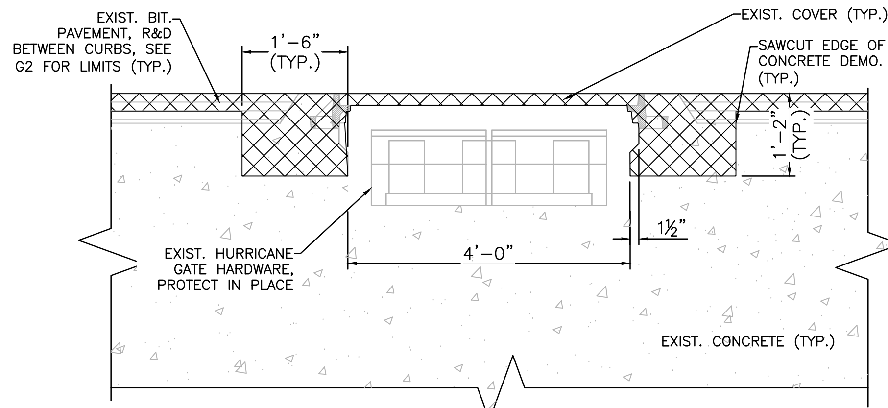
SECTION/DETAIL B SCALE: 3/4" = 1'-0"
