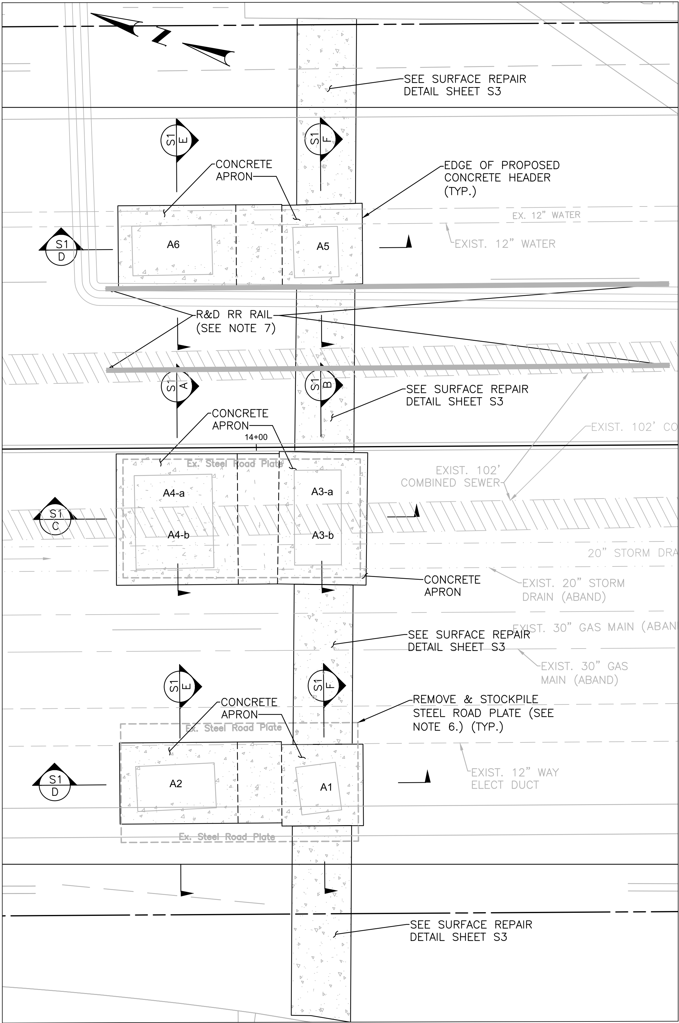
ALLENS AVENUE HURRICANE BARRIER GATE SCALE: 1" = 4'
