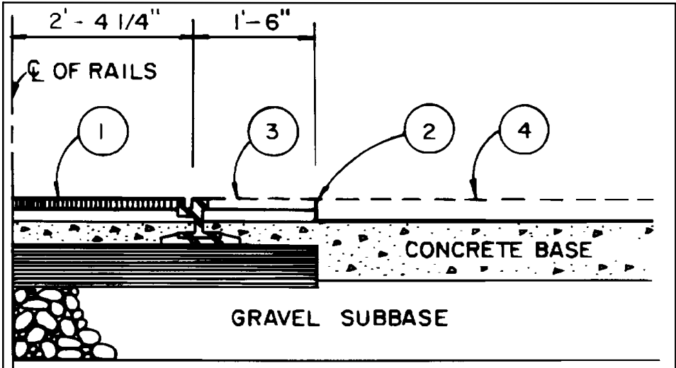
WORK SEQUENCE AT RAILROAD (IF NECESSARY) SCALE: NTS
