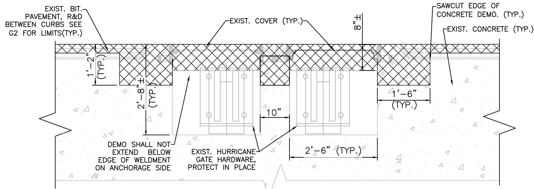
SECTION/DETAIL A SCALE: 3/4" = 1'-0"
