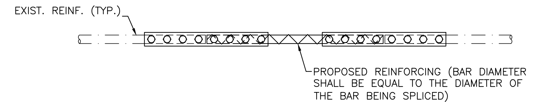
MECHANICAL COUPLER – OPTION 3
