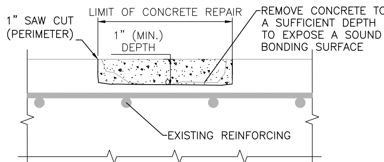
SURFACE REPAIR DETAIL B
