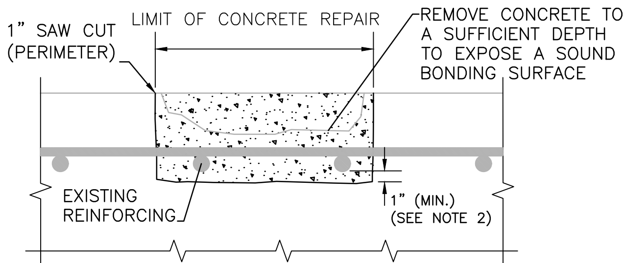
SURFACE REPAIR DETAIL A
