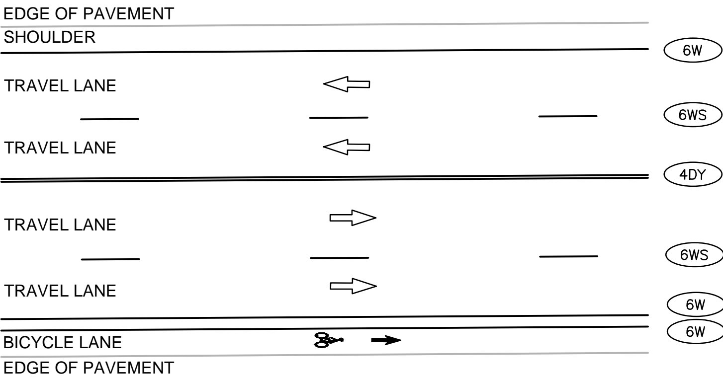
TYPICAL PAVEMENT MARKINGS SCALE: NTS SEE NOTE 4
