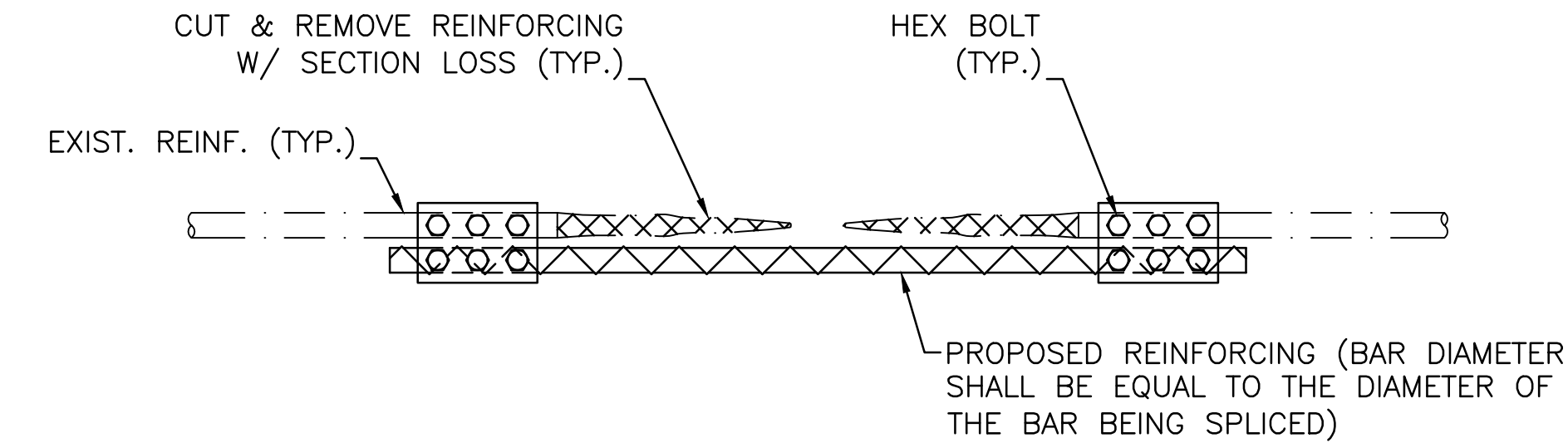
MECHANICAL COUPLER – OPTION 1
