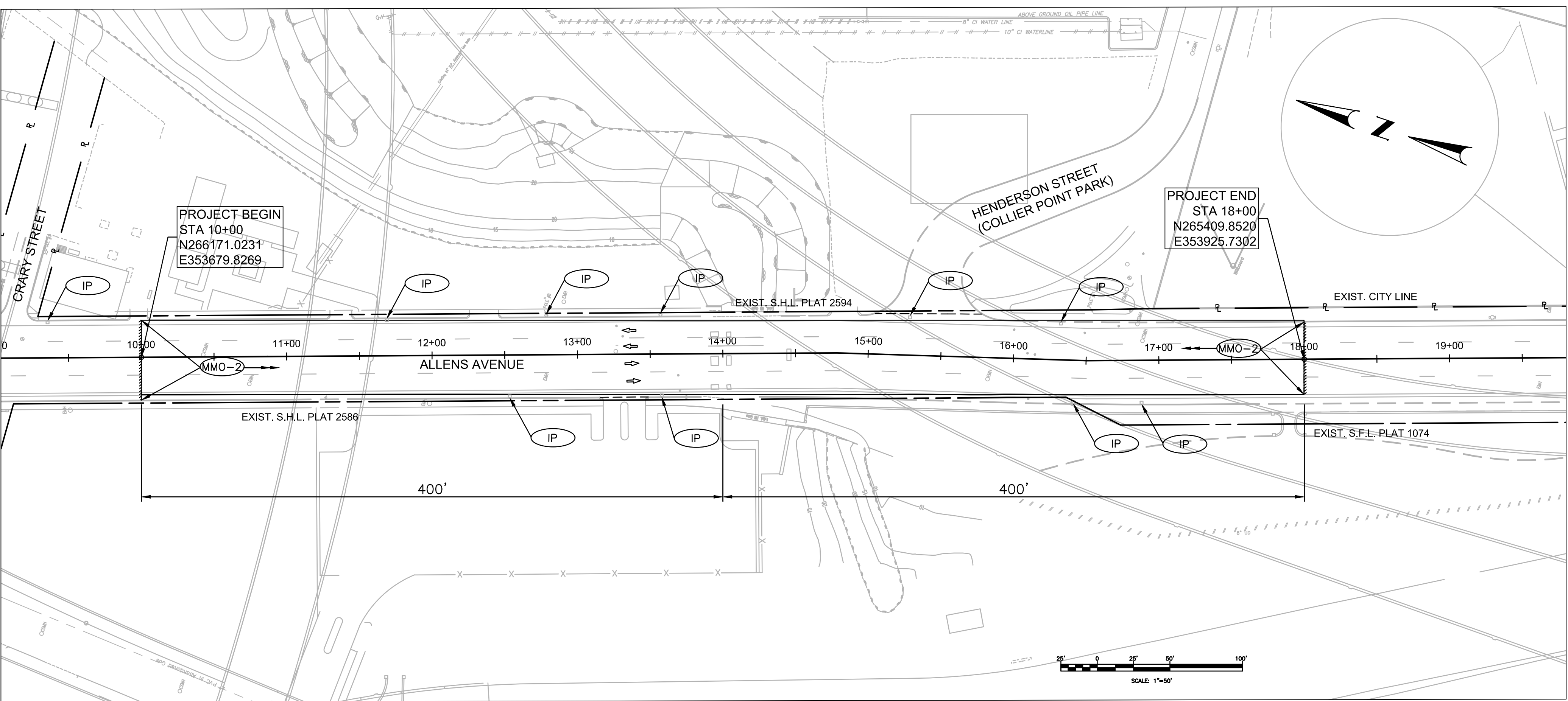
ALLENS AVENUE GENERAL PLAN SCALE: 1" = 50'
