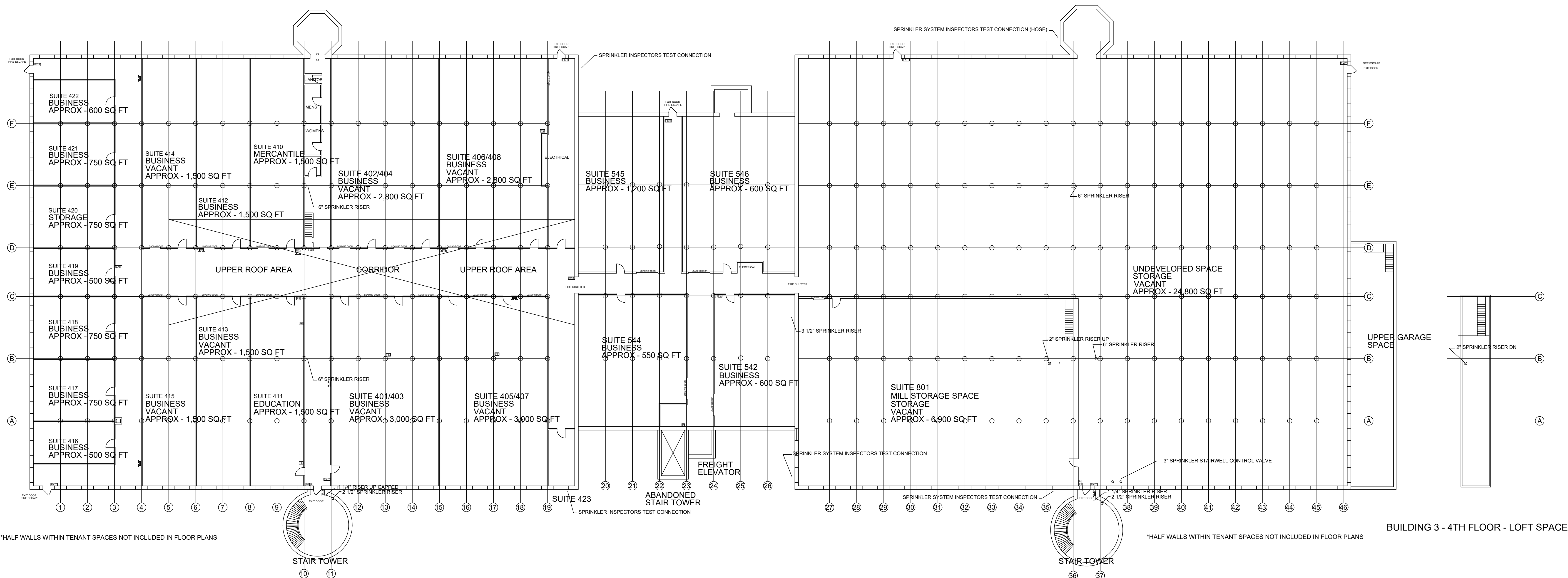
BUILDING 2 - 4TH FLOOR
