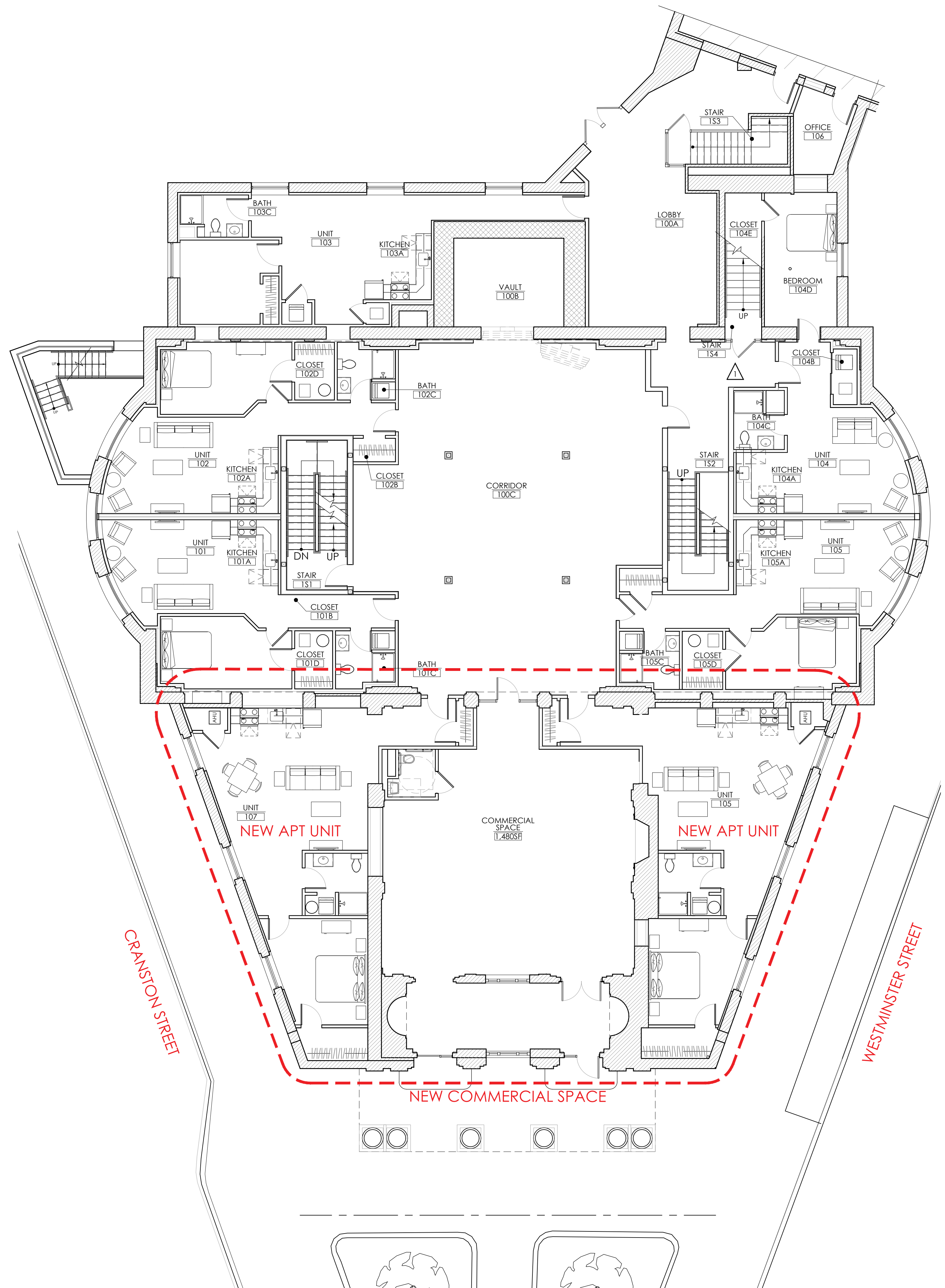
1 FIRST LEVEL FLOOR PLAN SCALE: 1/8"=1'-0"
