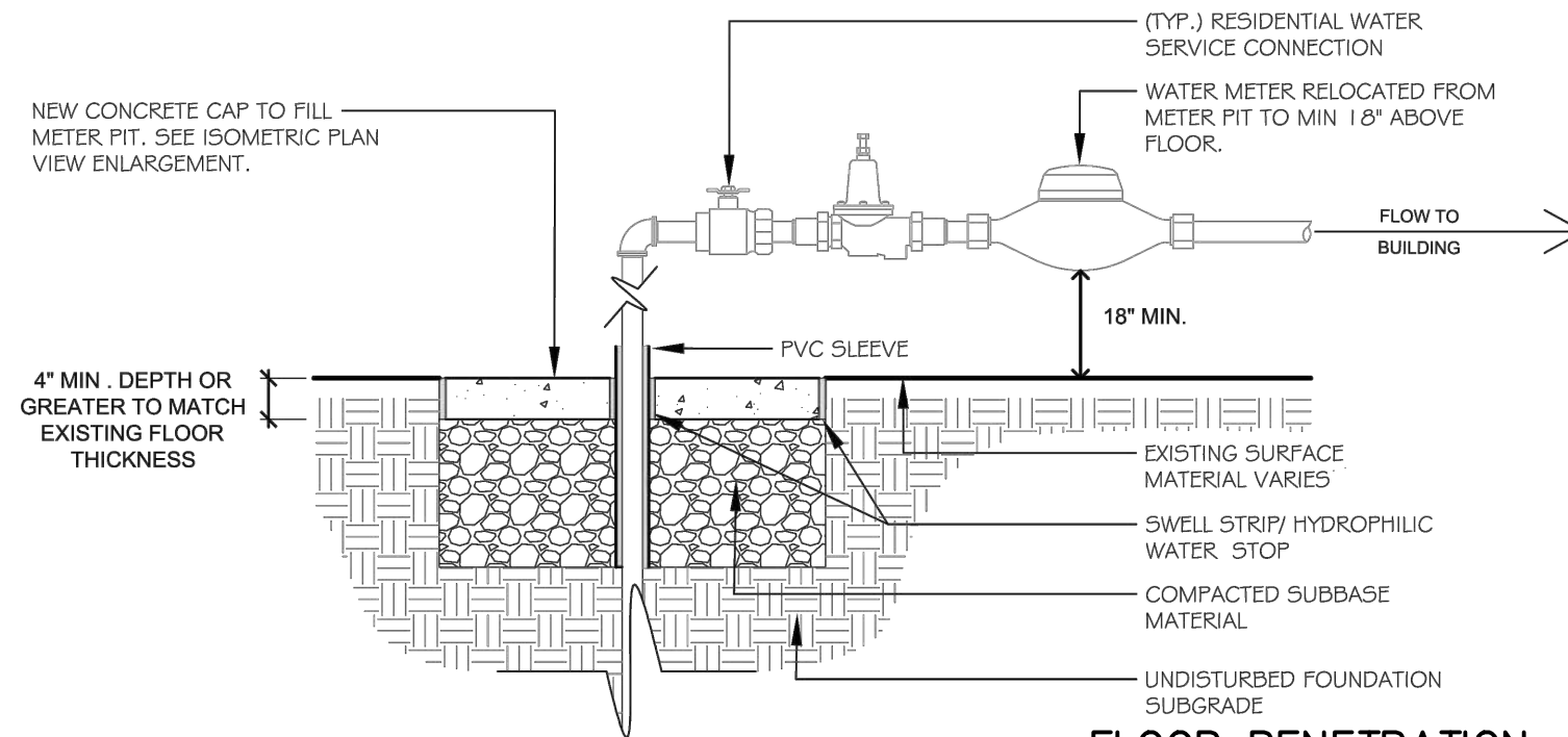
FLOOR PENETRATION DETAIL NTS
