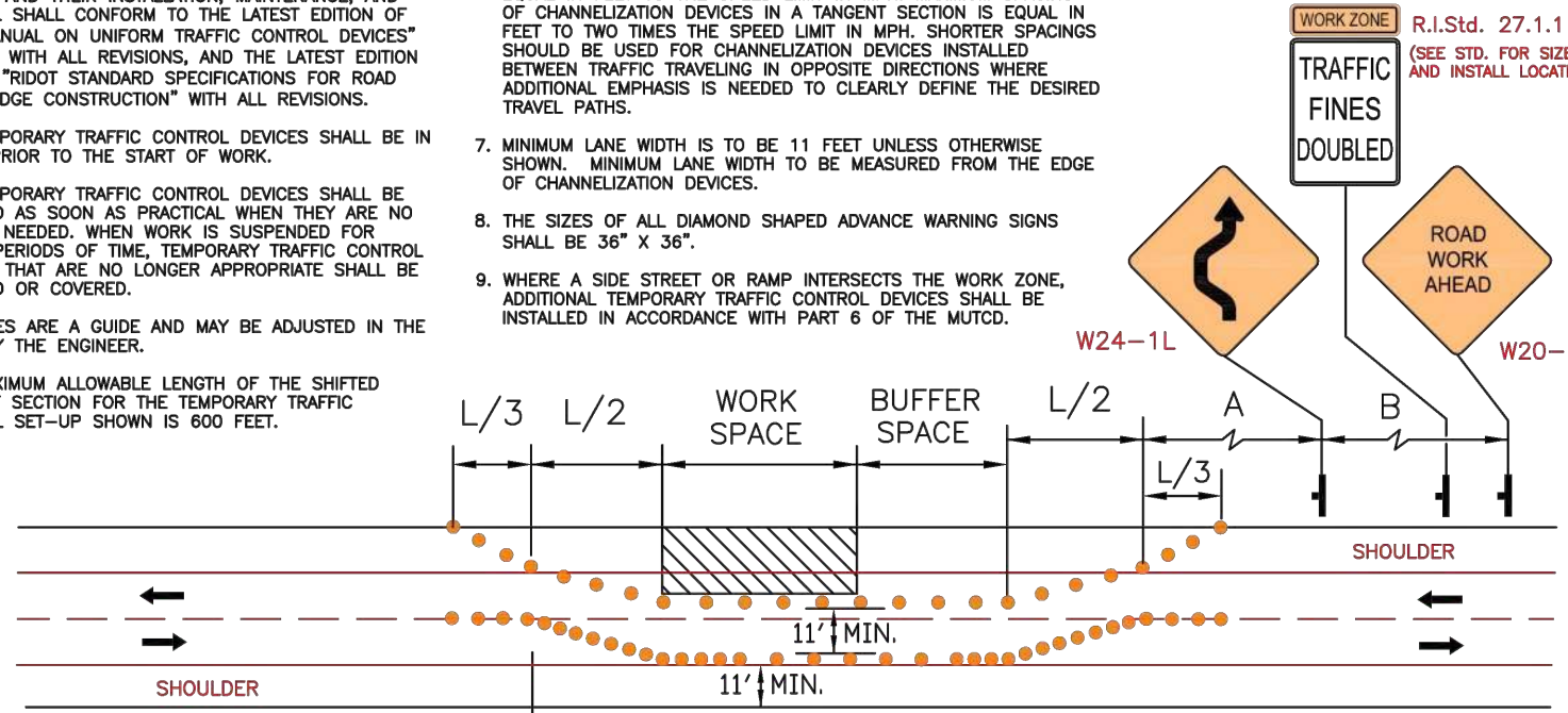
TAPER AND BUFFER LENGTHS
