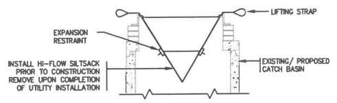
SILTSACK® AT CATCH BASIN NOT TO SCALE
