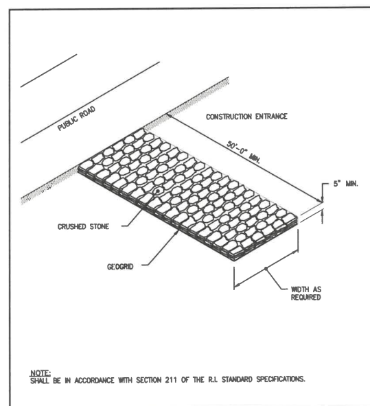
CONSTRUCTION ACCESS NOT TO SCALE
