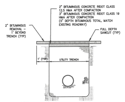
TRENCH RESURFACING NOT TO SCALE
