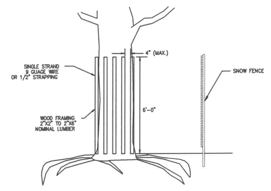
TREE PROTECTION NOT TO SCALE
