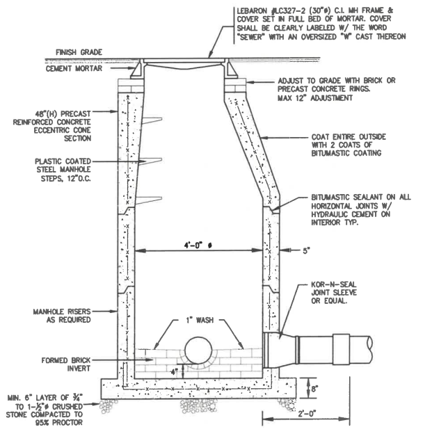
TRENCH SECTION (SEWER) NOT TO SCALE
