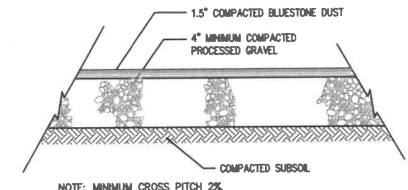
GRAVEL PATHWAY NOT TO SCALE
