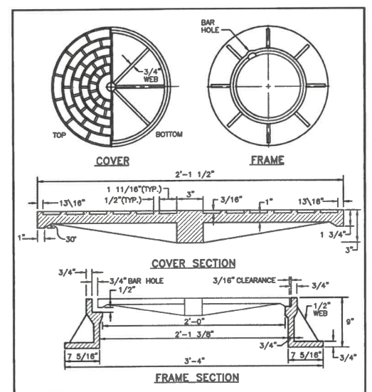
RHODE ISLAND DEPARTMENT OF TRANSPORTATION HEAVY-DUTY ROUND FRAME AND COVER R.I. STANDARD 6.2.1
