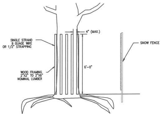
TREE PROTECTION NOT TO SCALE
