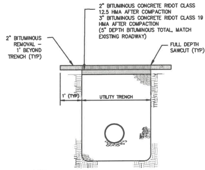
TRENCH RESURFACING NOT TO SCALE
