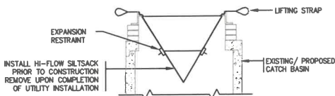
SILT SOCK® AT CATCH BASIN NOT TO SCALE
