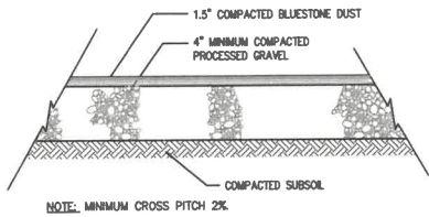
GRAVEL PATHWAY NOT TO SCALE
