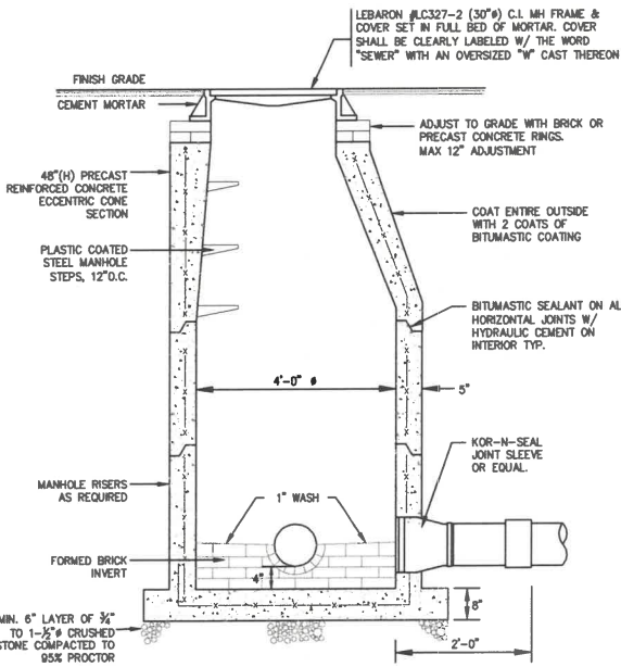
TRENCH SECTION (SEWER) NOT TO SCALE
