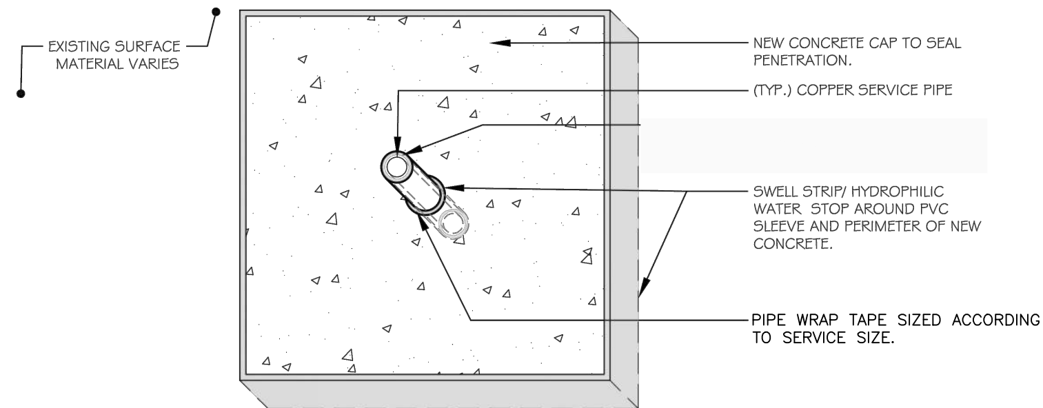
ISOMETRIC PLAN VIEW ENLARGEMENT NTS
