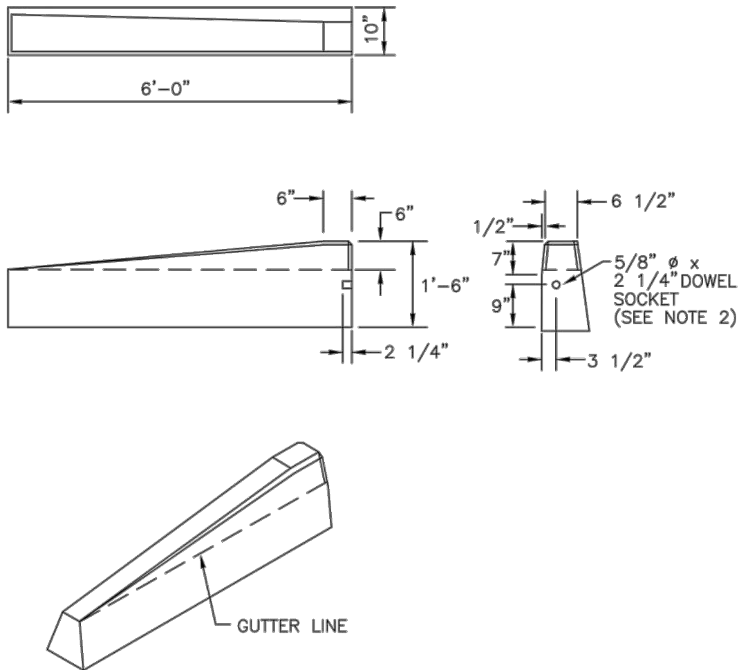
6'-0" PRECAST CONCRETE TRANSITION CURB NOT TO SCALE
