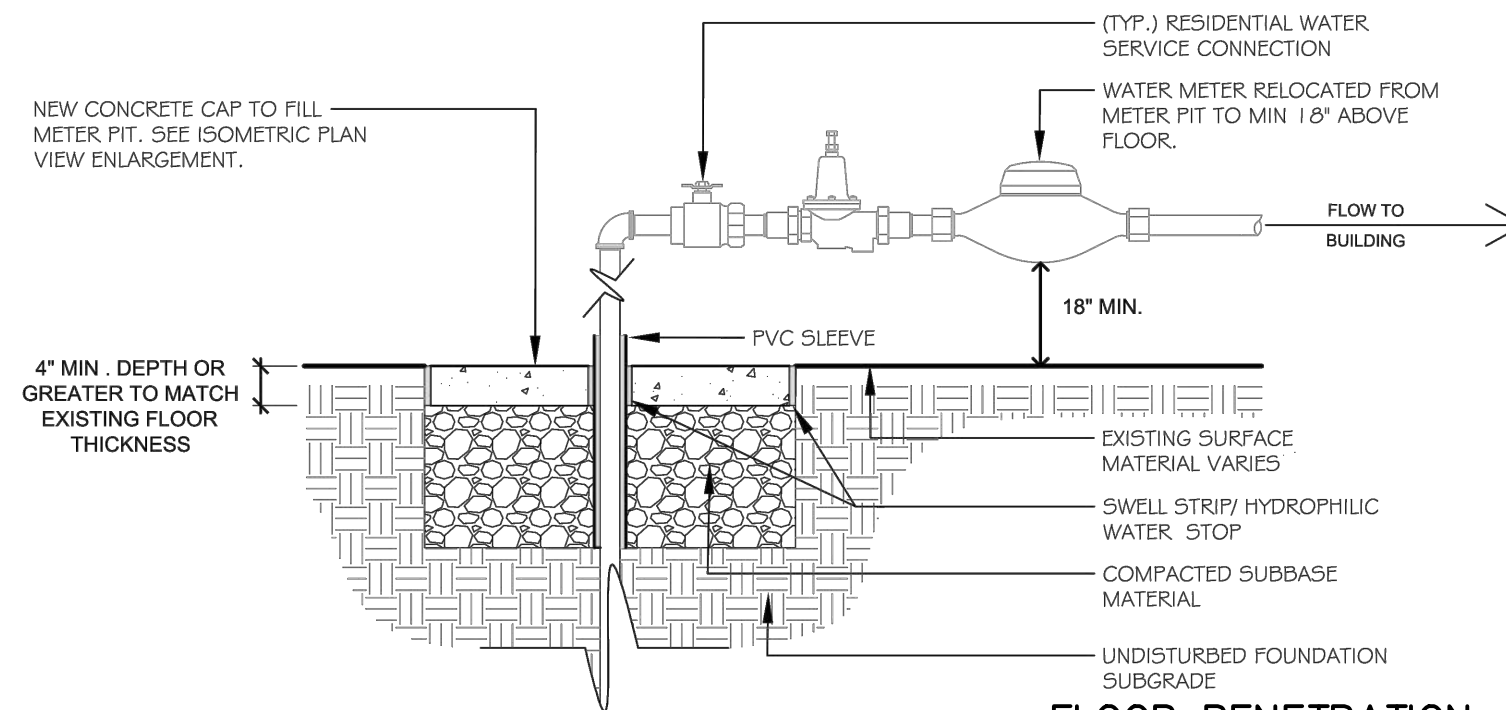
SECTION/ELEVATION NTS FLOOR PENETRATION DETAIL NTS
