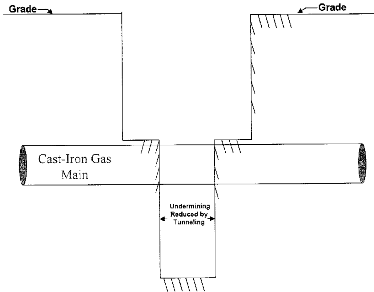
Elevation View
