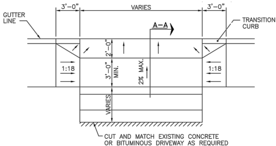
PLAN
