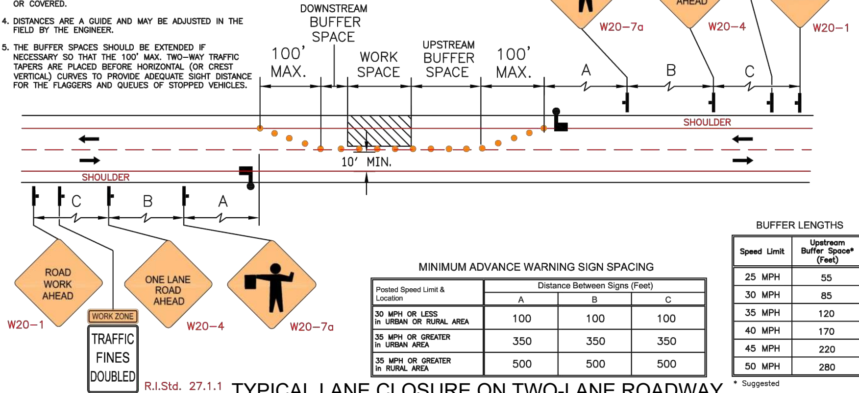
TYPICAL LANE CLOSURE ON TWO-LANE ROADWAY
