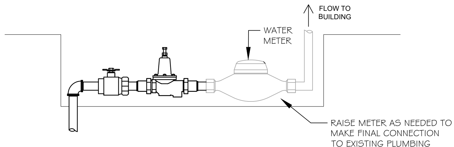
CONNECTION THROUGH EXISTING METER PIT NTS
