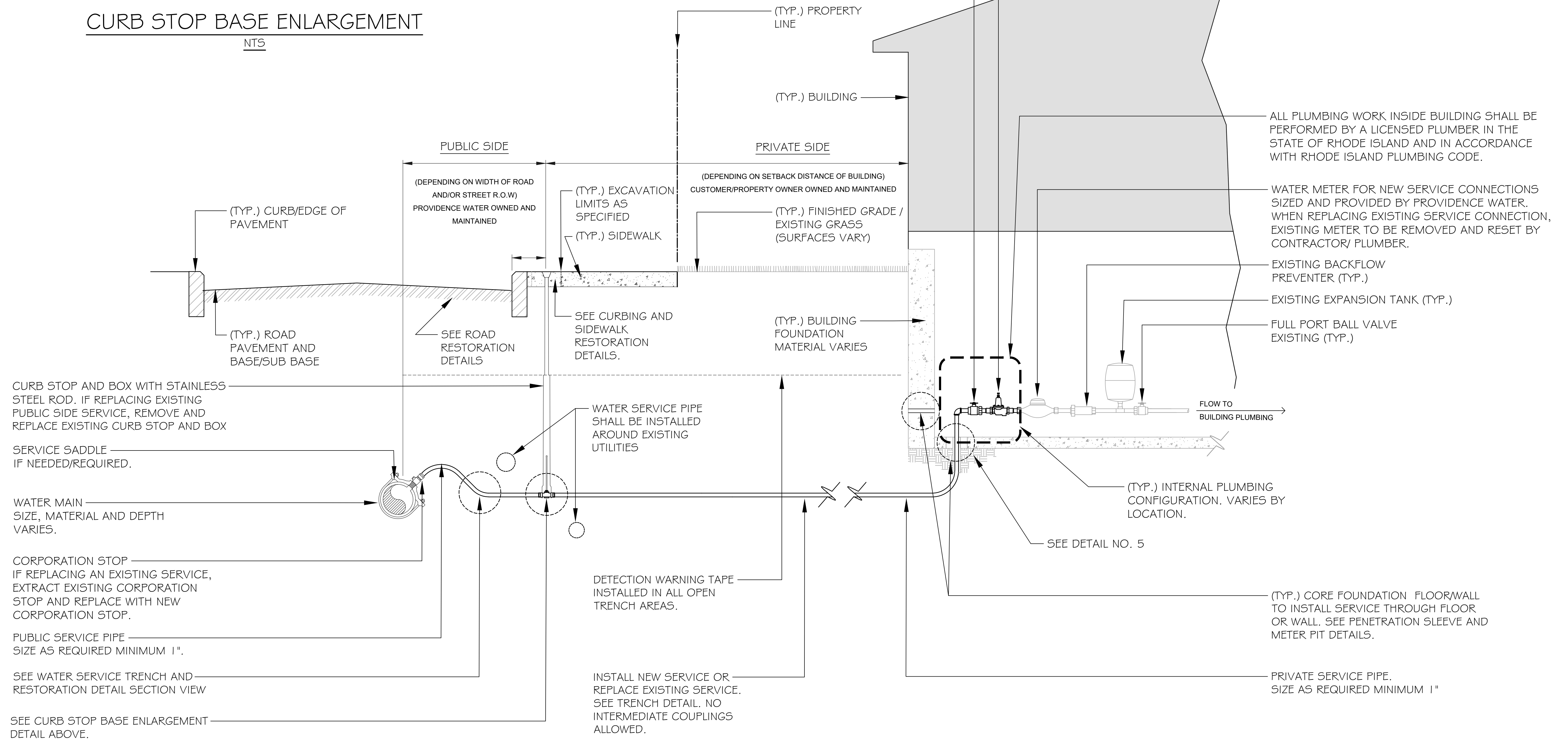
TYPICAL RESIDENTIAL WATER SERVICE CONNECTION - ELEVATION / SECTION VIEW NOT TO SCALE
