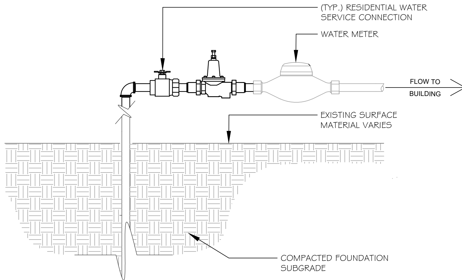
CONNECTION THROUGH EXISTING FINISHED FLOOR SECTION/ELEVATION NTS
