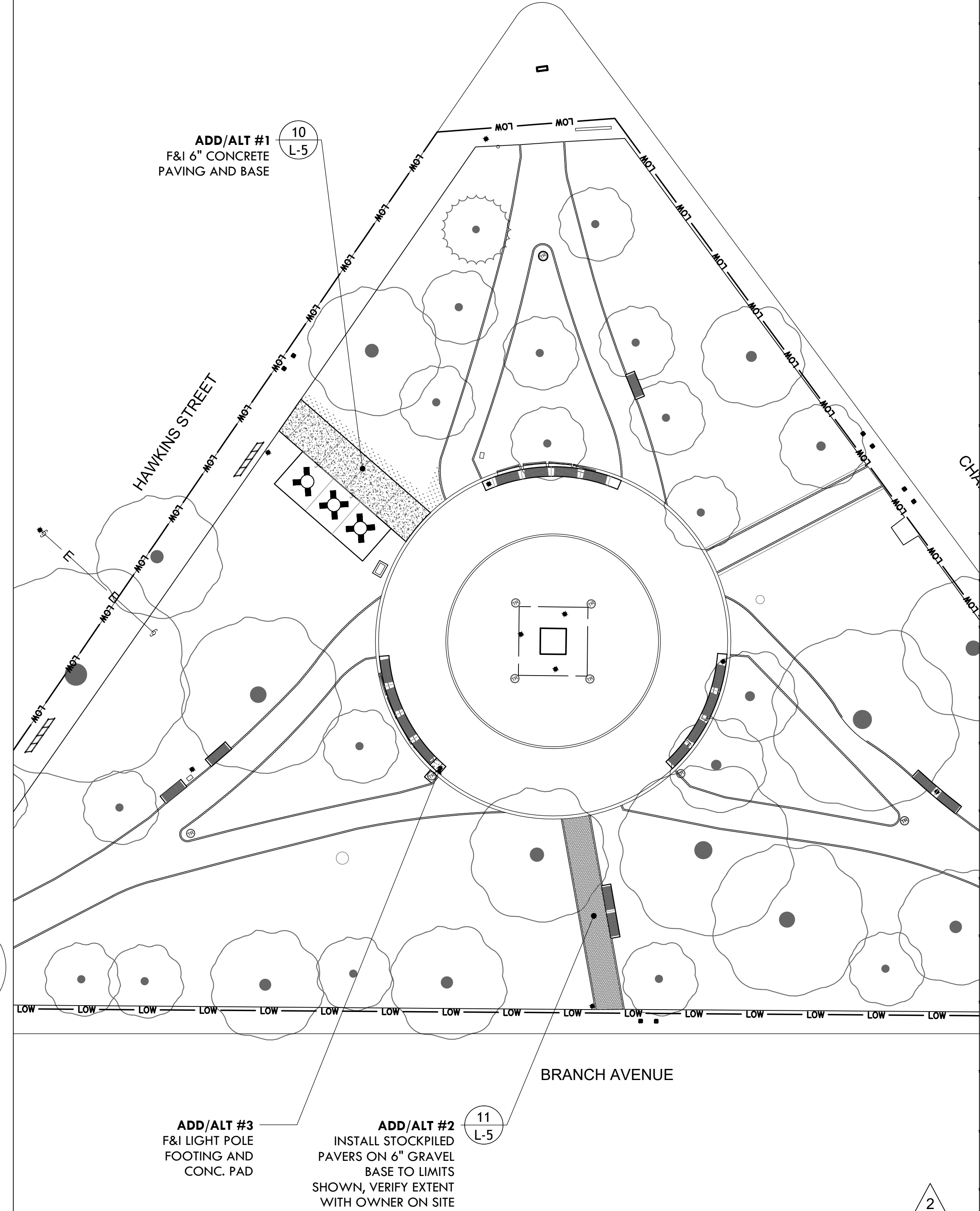
B ADD ALT ITEMS SCALE 1"=20'
