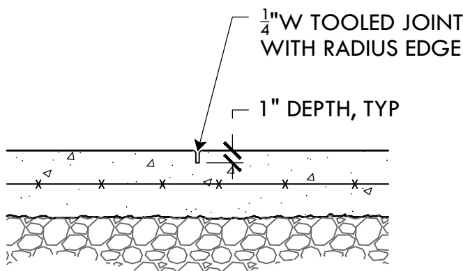
CONTROL JOINT
