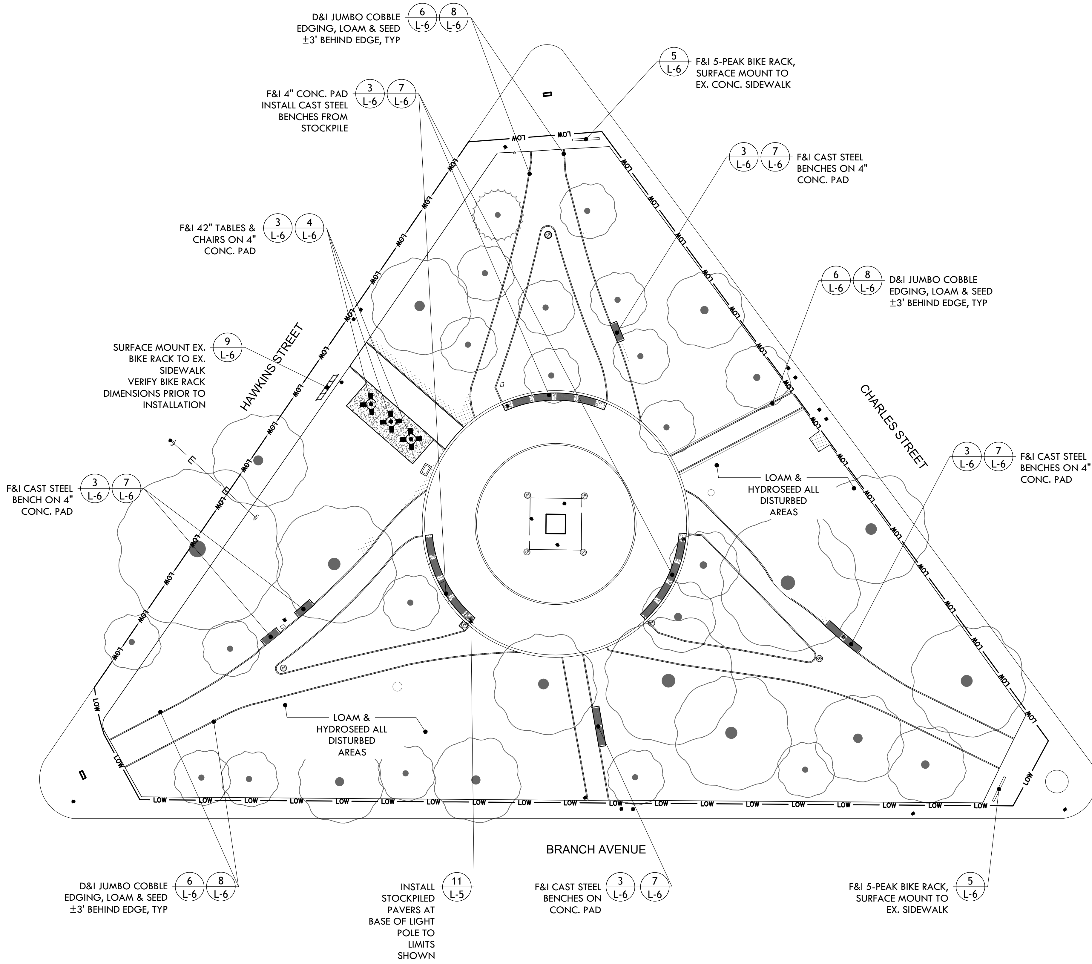
A BASE BID ITEMS SCALE 1"=20'
